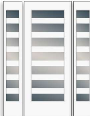
Door: 3/0 8/0 2680-010-C-X-SO4-7H Sidelites: 1/2 8/0 880-010-C-X-SO4-7H
