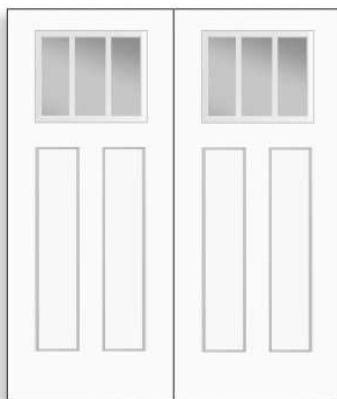
Door: 3/0 6/8 2215-010-2-031C (x2)
