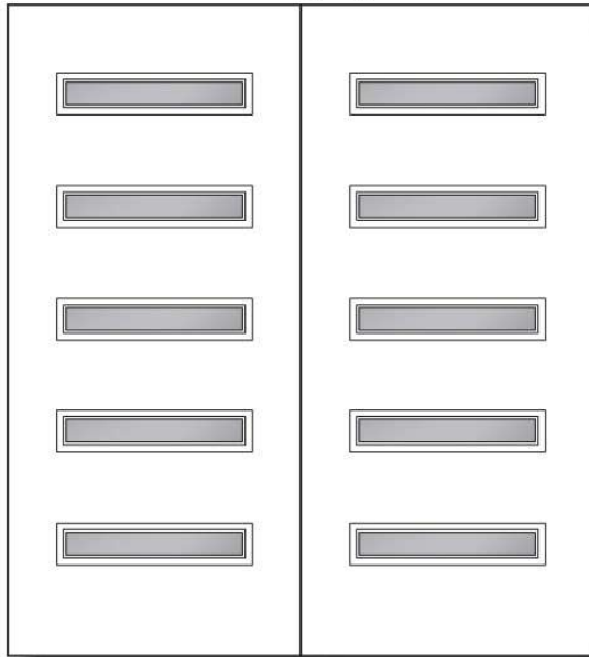
Door Glass Size: 22" x 3.5" (x5)
