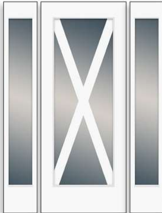
Door: 3/0 8/0 2680-010-C-X-SO4-1XBUK Sidelites: 1/2 8/0 880-010-C-X
