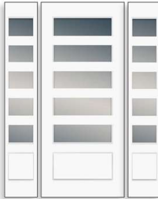
Door: 3/0 6/8 2648-010-C-1-SO4-5H Sidelites: 1/2 6/8 848-010-C-1-SO4-5H
