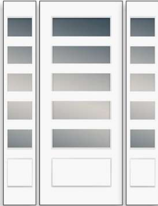
Door: 3/0 8/0 2664-010-C-1-SO3-5H Sidelites: 1/2 8/0 764-010-C-1-SO3-5H
