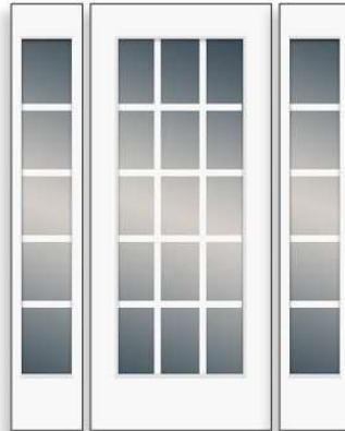
Door: 3/0 6/8 2664-010-C-X-SO-3W5H Sidelites: 1/2 6/8 764-010-C-X-SO-5H
